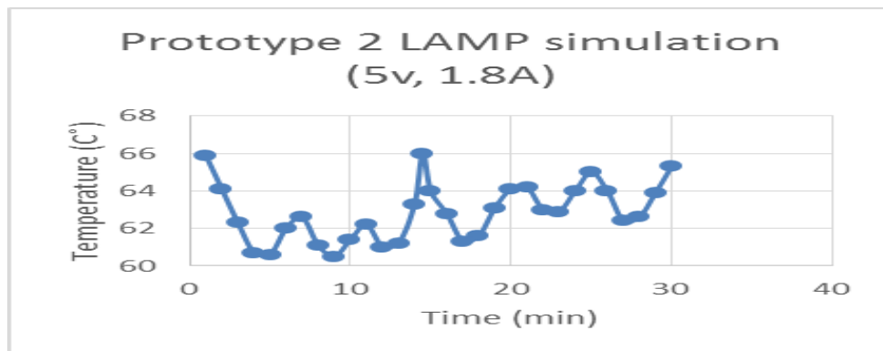
Figure 6: Graph of temperature change over time during a 30-minute PCR using prototype #2.
